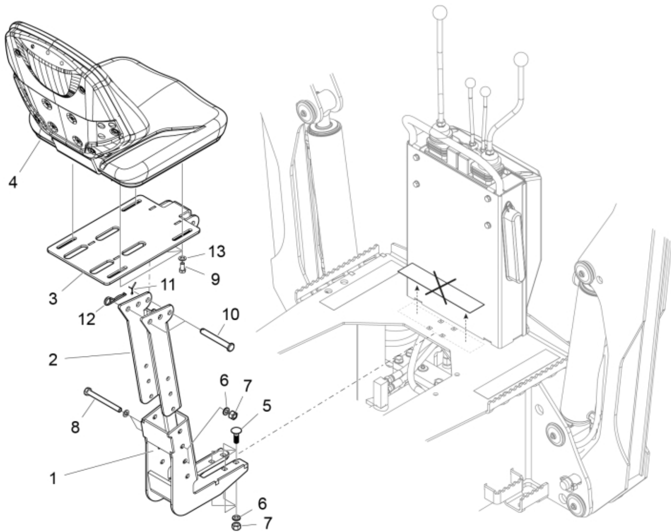
M 60117039 BH Seat
